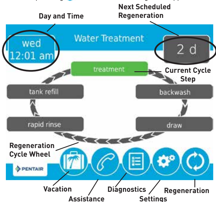
Figure 7 Home Screen
